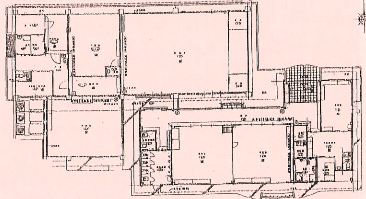
[園舎平面図]
